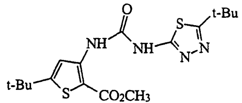
5-tert-Butyl-3-[3-(5-tert-butyl-[1,3,4]thiadiazol-2-yl)-ureido]-thiophene-2-carboxylic acid methyl ester
